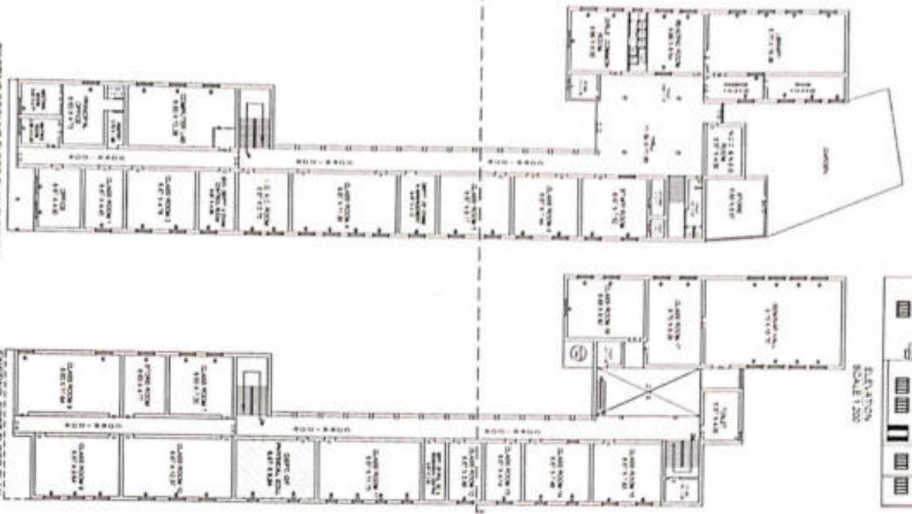
EXISTING GROUND FLOOR PLAN BLOCK (A) SCALE 1:200
